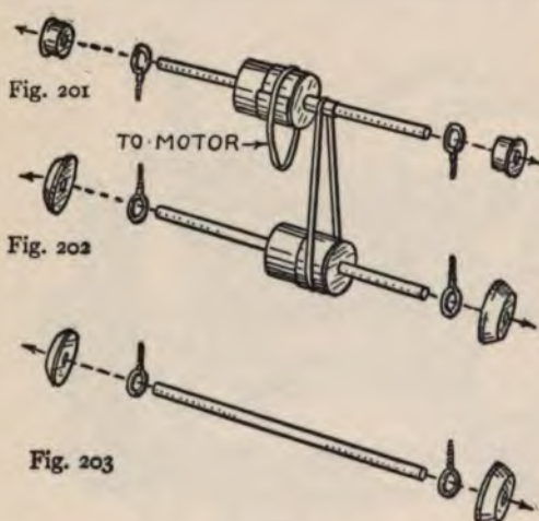
FIGS. 201-203. — Details of Axle and Belt Shaft.
